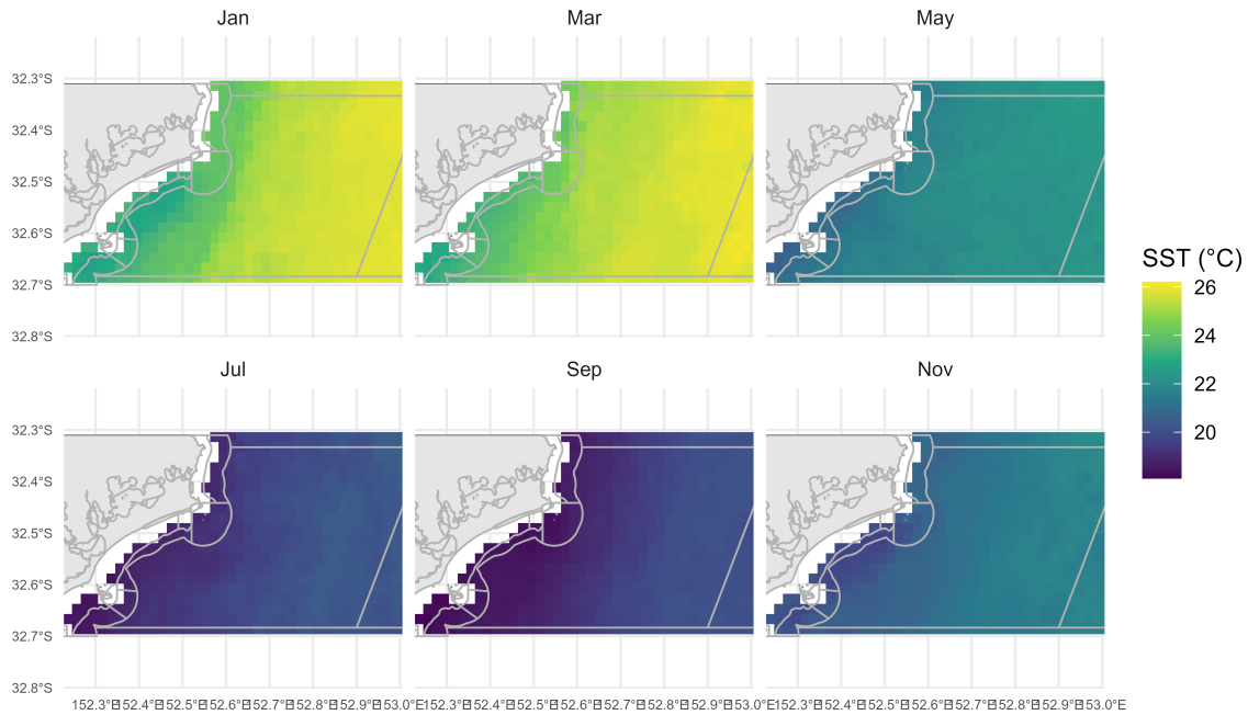
Figure C.3: Sea surface temperature at the scale of the GMP. Heatmap values represent high (yellow) and low (blue) bimonthly sea surface temperature (SST). Grey polygons represent State spatial management and Australian Marine Park boundaries.
