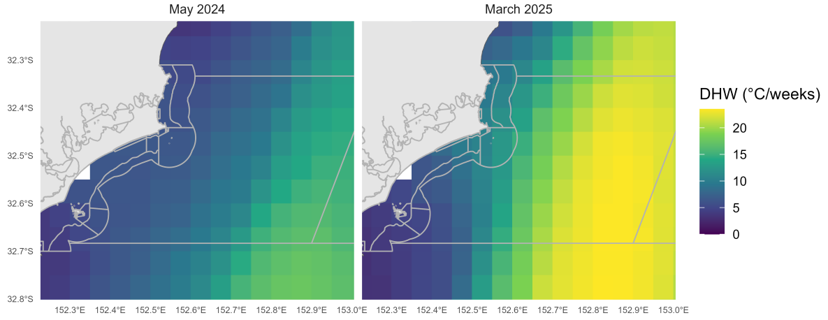
Figure C.4: Maximum Degree Heating Weeks at the scale of the GMP. Heatmap values representing high (yellow) and low (blue) monthly Degree Heating Weeks (DHW) for the two most recent marine heatwave periods on record. Grey polygons represent State spatial management and Australian Marine Park boundaries.
