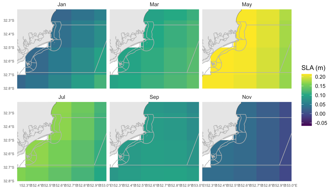
Figure C.2: Sea level anomaly, as an index of upwelling, at the scale of the GMP. Heatmap values represent high (yellow) and low (blue) bimonthly sea level anomaly (SLA). Grey polygons represent State spatial management and Australian Marine Park boundaries.
